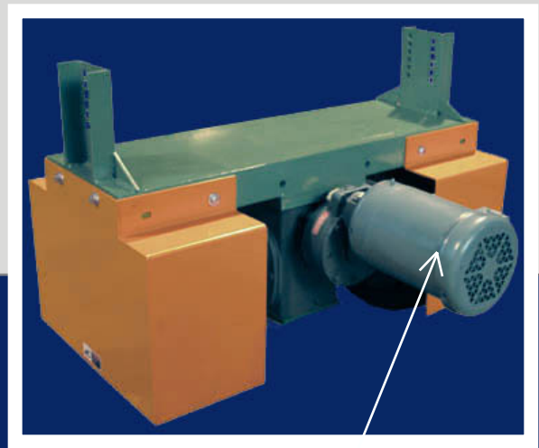
Heavy Duty Motor and Reducer 230/460 Volt, 3 Phase or 120 Volt, 1 Phase Drives
